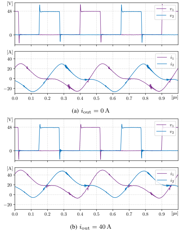
Fig. 10: Measured waveforms at f_s = 2 MHz with a 5 ns dead-time. Note: The current-sensor is operating close to its maximum bandwidth and has deskewing applied.
