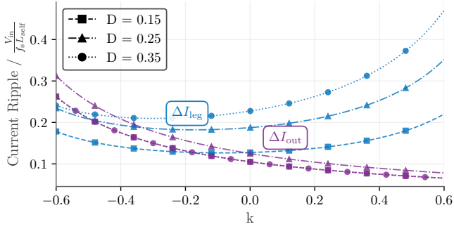
Fig. 5: Peak-to-peak leg and output current ripple in dependency of the coupling factor for different duty cycles D . Note: For D = 0.15 and D = 0.35 the output current ripple is identical so the curves overlap.
